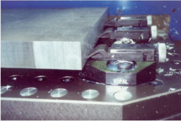
Machining of an aluminium plate with mini driving clamps on special supports
